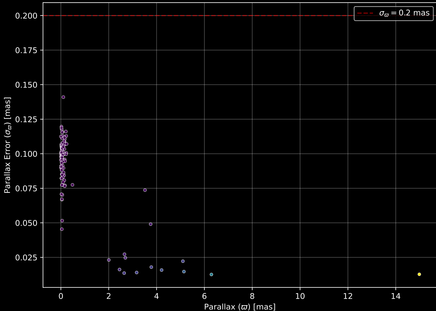
APOGEE DR17 Field: [FORNAX] Parallax Quality (n= 127)
