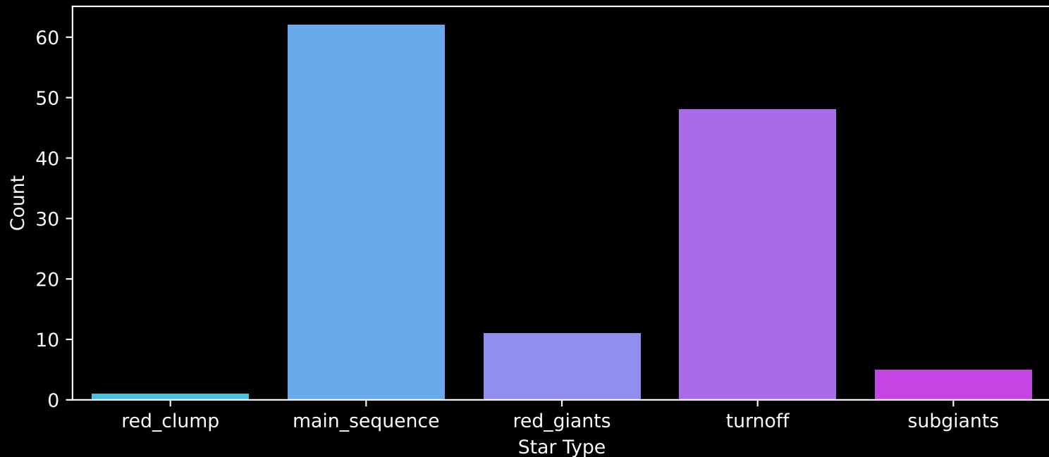
APOGEE DR17 Field: [FORNAX] Count plot of Star Type
