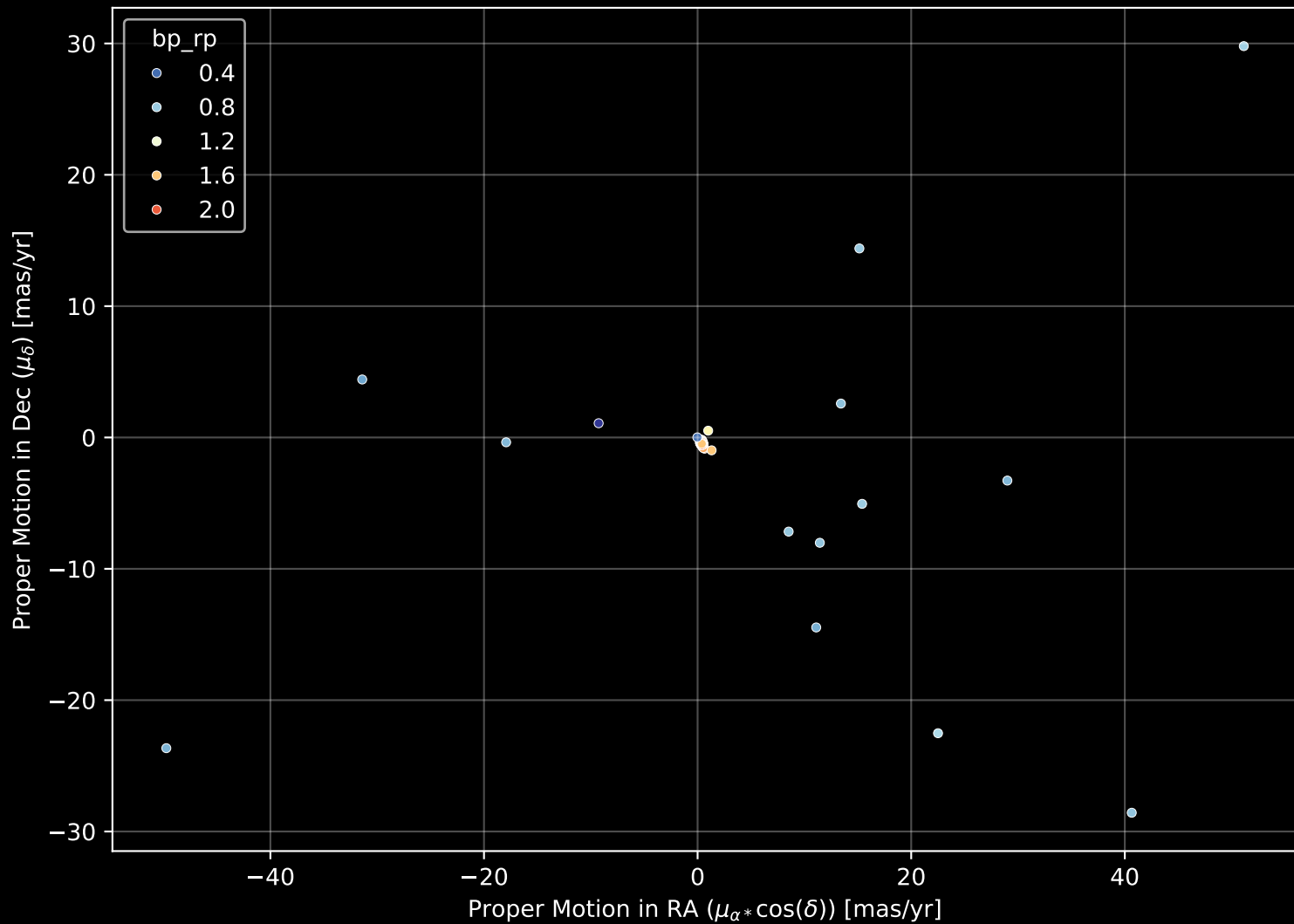
APOGEE DR17 Field: [FORNAX] Proper Motion Diagram (n= 127)
