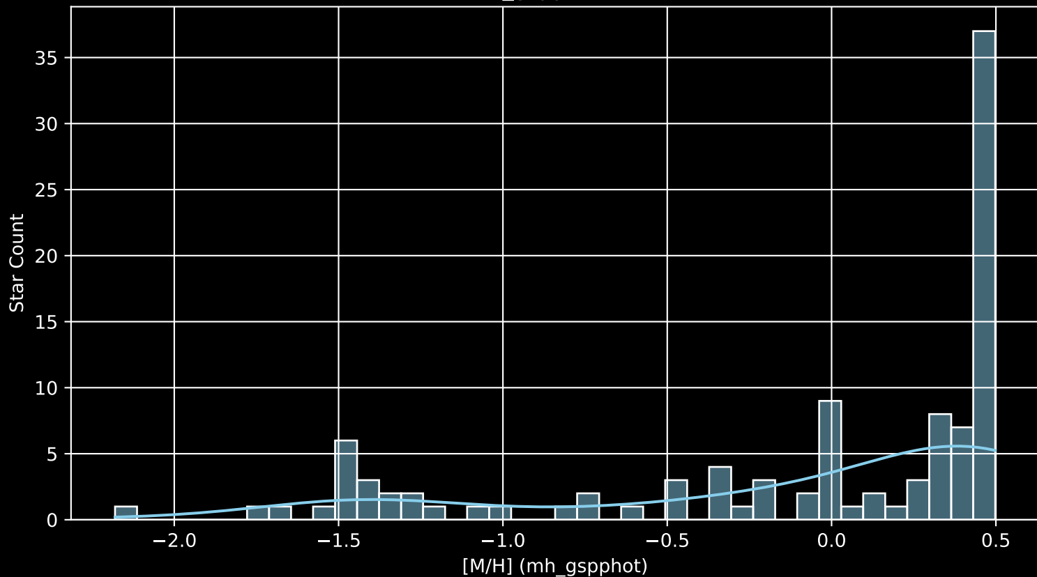
APOGEE DR17 Field: [FORNAX [M/H] (mh_gspphot) (n= 105)
