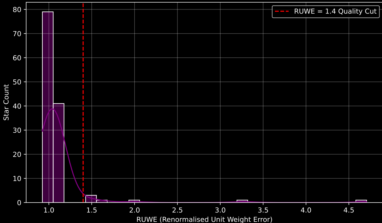
GAPOGEE DR17 Field [FORNAX] RUWE Distribution (n= 127)
